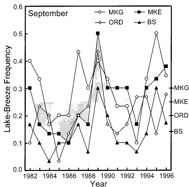
FIG. 6. Sep lake-breeze frequency for Milwaukee, WI (MKE), Muskegon, MI (MKG), Chicago, IL (ORD), and both shores (BS) from 1982 to 1996. The average Sep frequency for each curve is shown on the right vertical axis. Shaded regions represent example of extended time periods when MKE frequency is above or below average.
