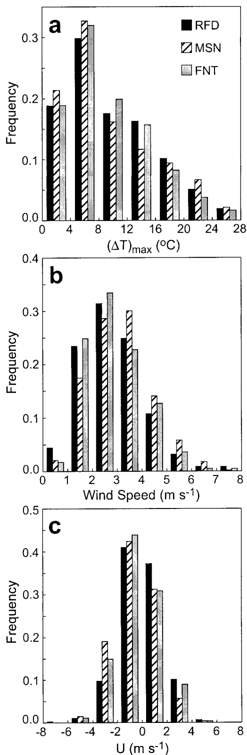
FIG. 7. Observed frequency of (a) maximum air-lake temperature difference (\Delta T)_{\max} , ^{\circ}\text{C} , (b) average daytime (1000–1600 LST) wind speed ( \text{m s}^{-1} ), and (c) average daytime shore-perpendicular wind speed U ( \text{m s}^{-1} ) during lake-breeze events for Rockford, IL (RFD), Madison, WI (MSN), and Flint, MI (FNT).
