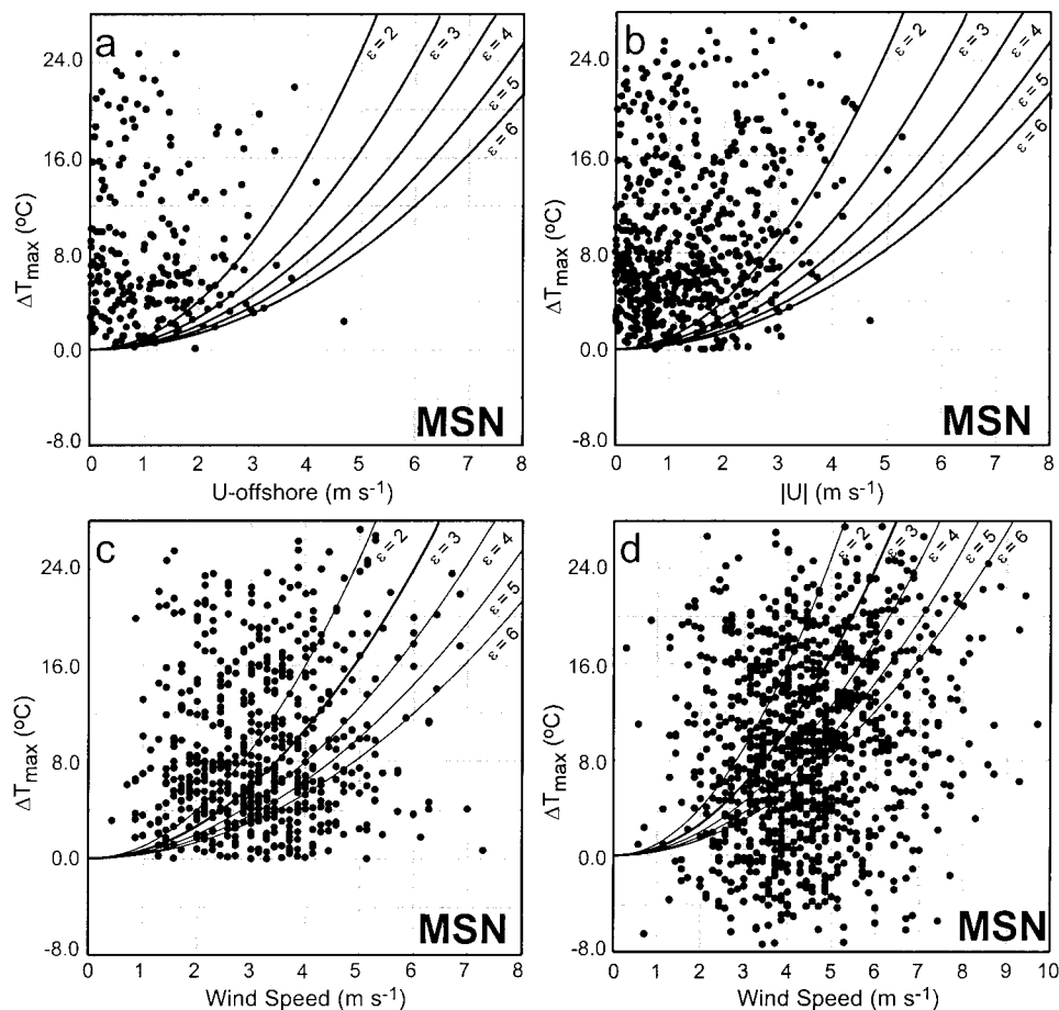
FIG. 9. Lake-breeze index \varepsilon calculated using data from Madison, WI (MSN), and NOAA buoy 45007. Index for lake-breeze days was determined using maximum air-lake temperature difference ( \Delta T_{\max} (°C)) and (a) shore-perpendicular wind component U during offshore gradient flow ( \text{m s}^{-1} ), (b) |U| for both offshore and onshore gradient flow ( \text{m s}^{-1} ), and (c) wind speed ( \text{m s}^{-1} ). (d) Index for non-lake-breeze days was calculated using ( \Delta T_{\max} (°C)) and MSN wind speed ( \text{m s}^{-1} ). Shown on each panel are curves for critical values of \varepsilon = 2, 3, 4, 5 , and 6 .
