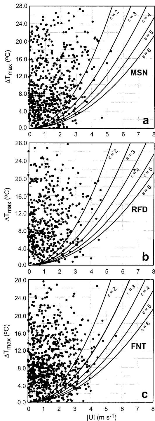
FIG. 10. Lake-breeze indices \varepsilon calculated using data from (a) Madison, WI (MSN), (b) Rockford, IL (RFD), (c) Flint, MI (FNT), and NOAA buoy 45007. Values of index were calculated from maximum air–lake temperature difference (\Delta T)_{\max} ( ^\circ\text{C} ) and shore-perpendicular wind component |U| for both offshore and onshore gradient flow ( \text{m s}^{-1} ). Shown on each panel are curves for critical values of \varepsilon = 2, 3, 4, 5 , and 6 .
