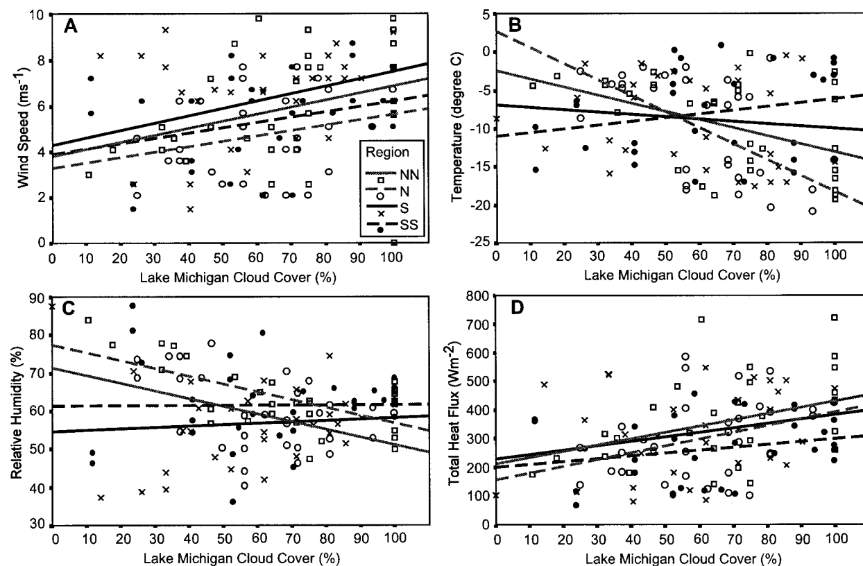
FIG. 5. Scatterplots showing the relationship between the percentage of Lake Michigan covered by lake-effect clouds and total flux, upwind air temperature, upwind relative humidity, and wind speed. A regression line, derived using least squares method, is given for each of the four regions over Lake Michigan studied.
