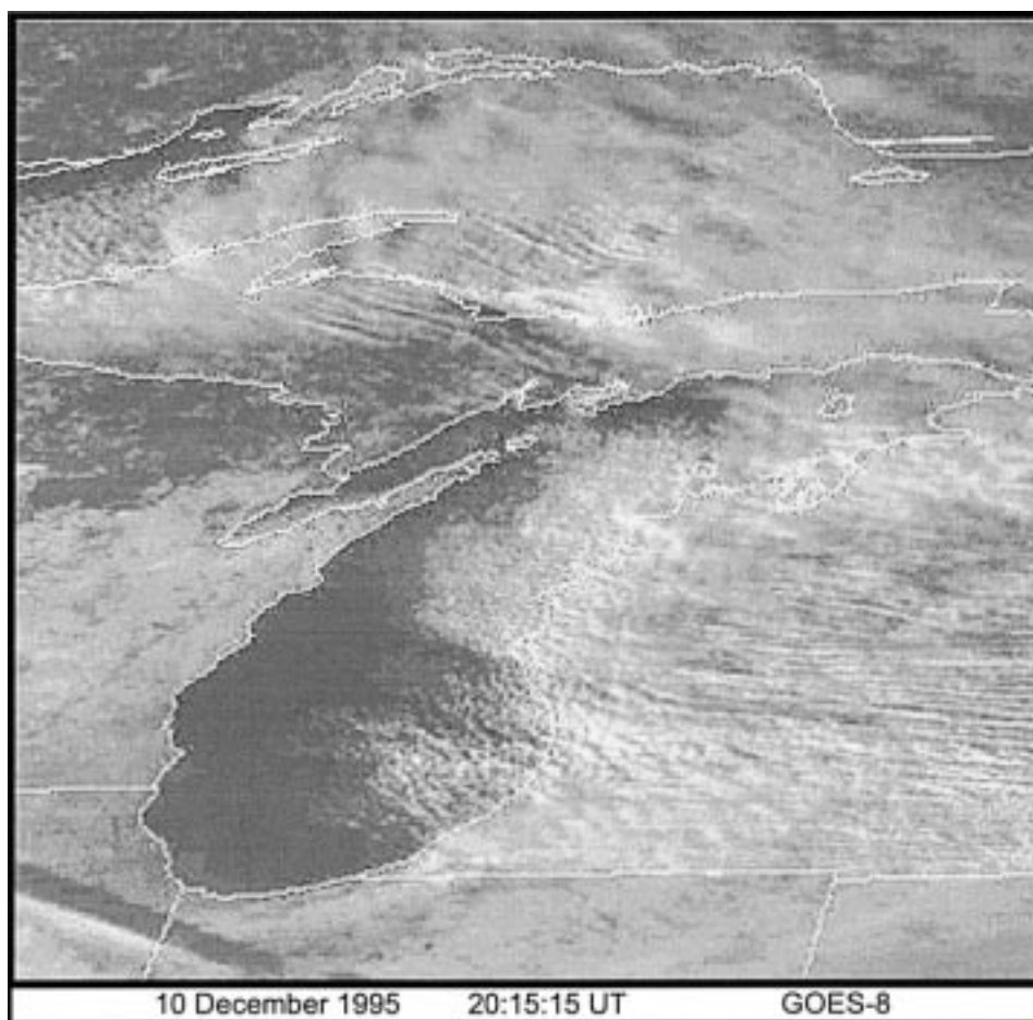
FIG. 1. GOES-8 visible satellite image of lake-effect clouds over Lake Michigan on 10 December 1995 at 2015 UTC. (Image courtesy of CIRA, Fort Collins, CO.)
